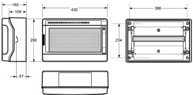
Armario / Enclosure - Ref. Item 39018
