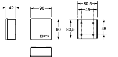
Caja estanca IP55 / Sealed box IP55 - Ref. Item 3062
