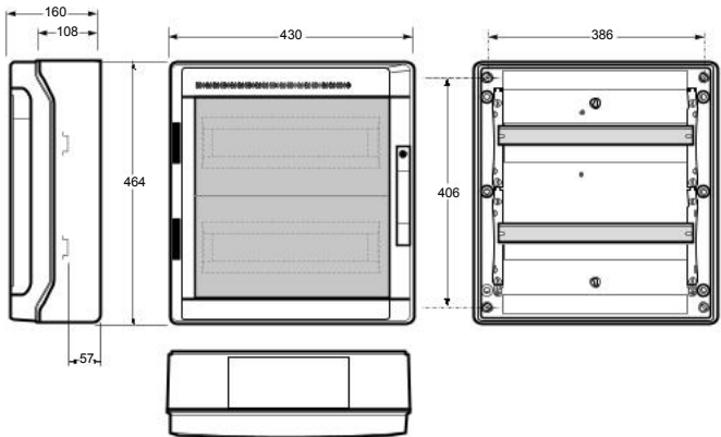
Armario / Enclosure - Ref. Item 39036
