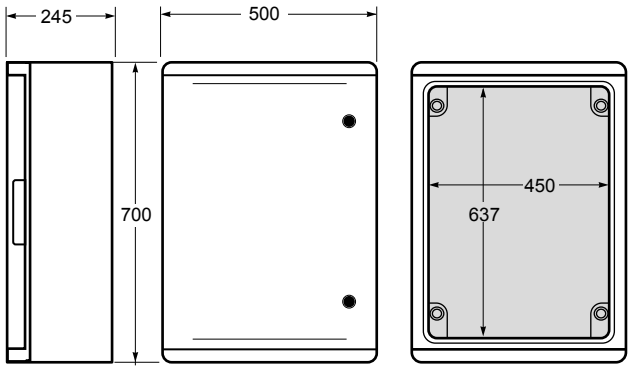
Armario / Enclosure - Ref. Item 39168-T / 39168
